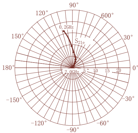
S 21e -FREQUENCY CONDITION: V CE =5V, I C =20mA
