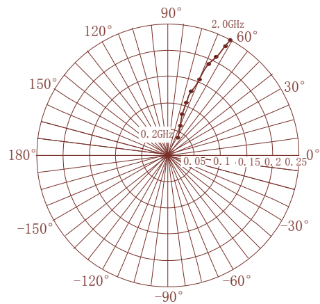
S 12e -FREQUENCY CONDITION: V CE =5V, I C =20mA
